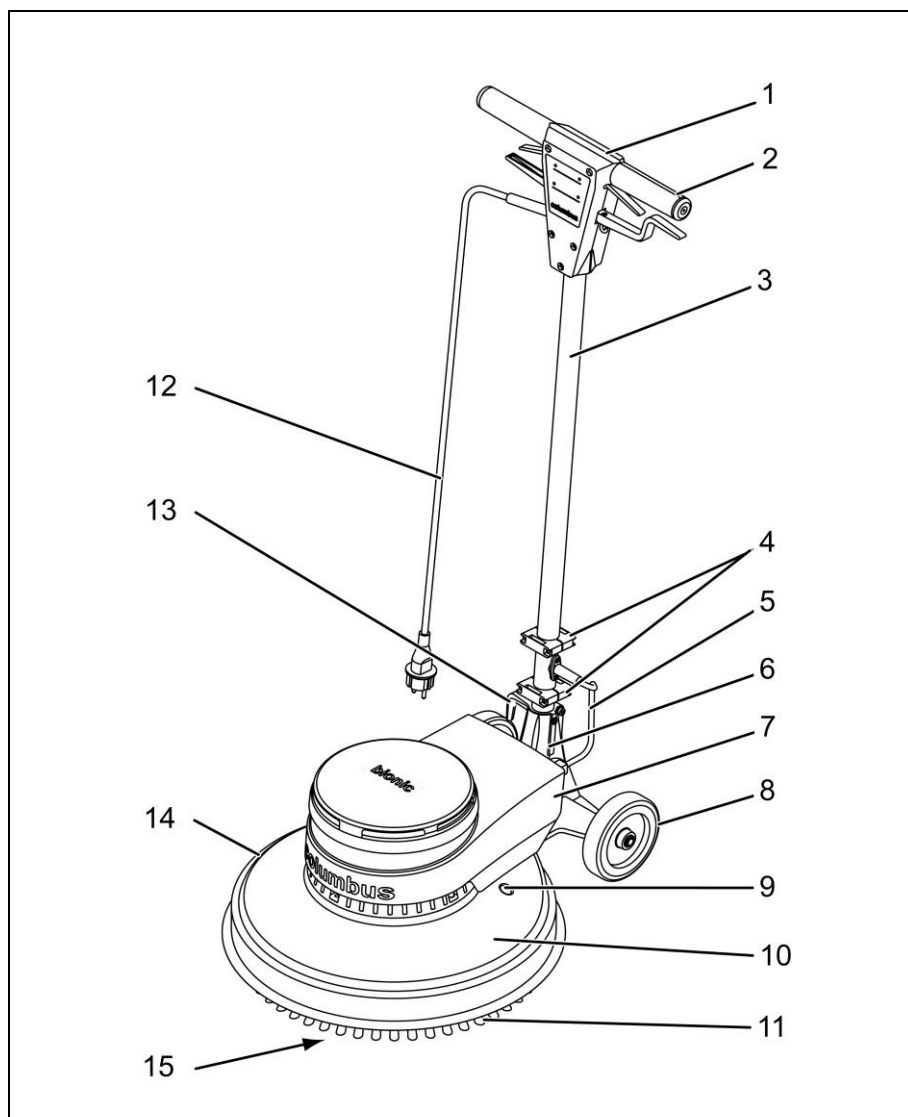
Fig. 1: Appliance overview
