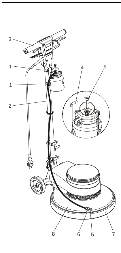
Fig. 7: Assembling the spray device
