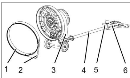
Fig. 10: Assembling the vac unit
