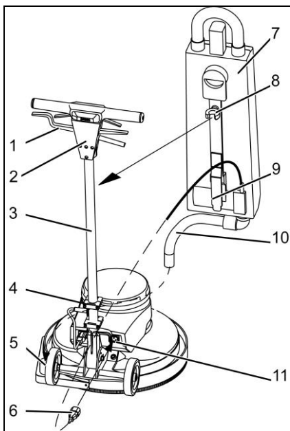
Fig. 12: Assembling the suction bin
