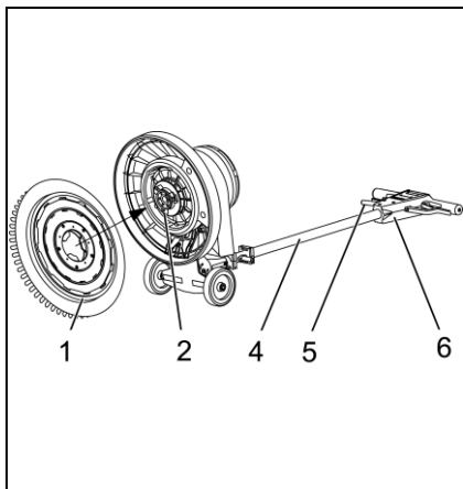
Fig. 16: Manual tool attachment
