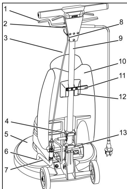
Fig. 8: Assembling the fluid tank
