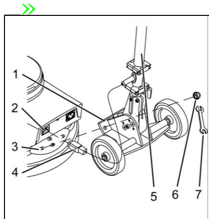
Fig. 5: Assembly of guide bar
