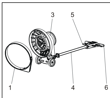
Fig. 10 Assembling the vac unit
