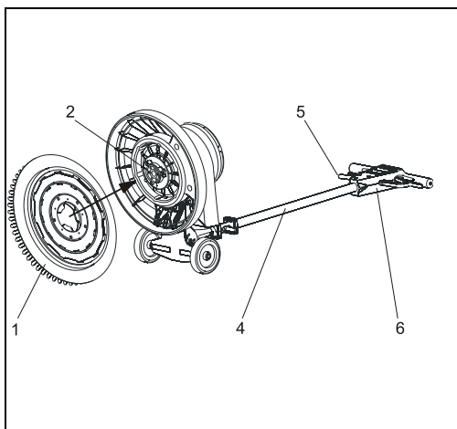
Fig. 16 Manual tool attachment
