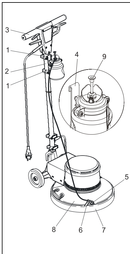
Fig. 7 Assembling the spray device
