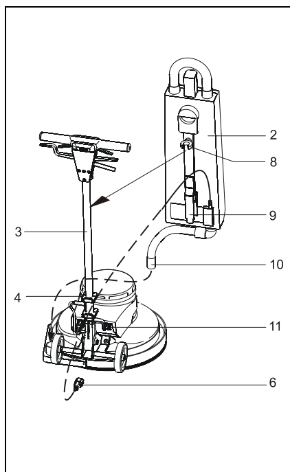
Fig. 12 Assembling the suction bin
