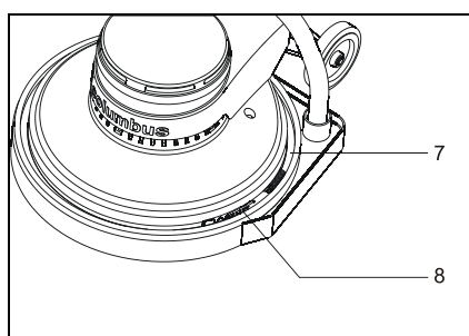
Fig. 11 Assembling the suction ring
